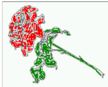
Figure 12: Caption vertically centered right beside the float with a caption width of the height of the image and a rotation of the caption and the object.
